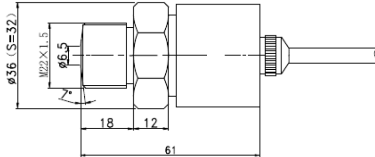
MRT22 with M22*1.5 port connector
